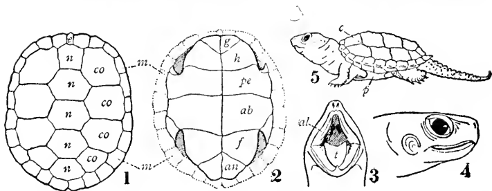
FIG. 3. Topography of a turtle. e , nuchal plate; n , neural plates; co , costal plates; m , marginal plates; g , gular plates; h , humeral plates; pe , pectoral plates; ab , abdominal plates; f , femoral plates; an , anal plates; c , carapace; p , plastron; al , alveolar surface; t , tongue.
